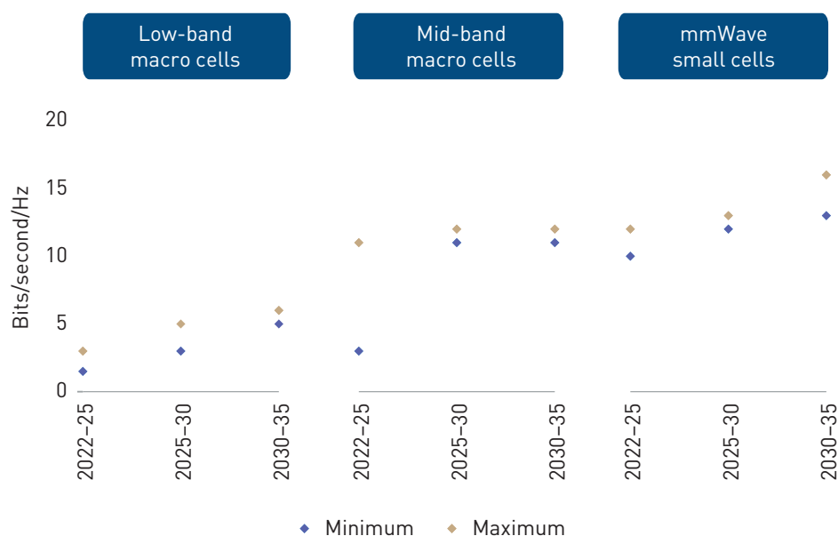
FIGURE C.4: INCREASE IN APPROXIMATE SPECTRAL EFFICIENCY PER CELL OVER TIME
